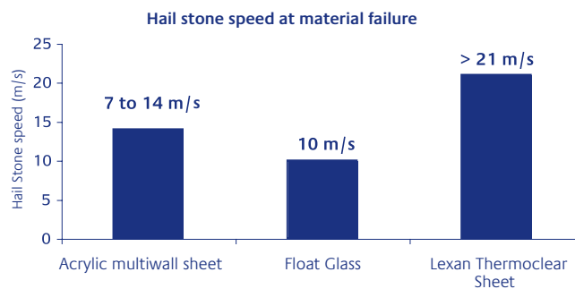
Figure 3: Impact Resistance
