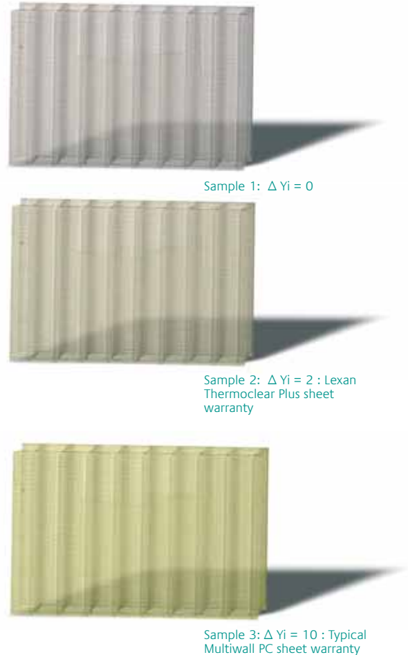
Figure 1: Yellowness index through weathering
