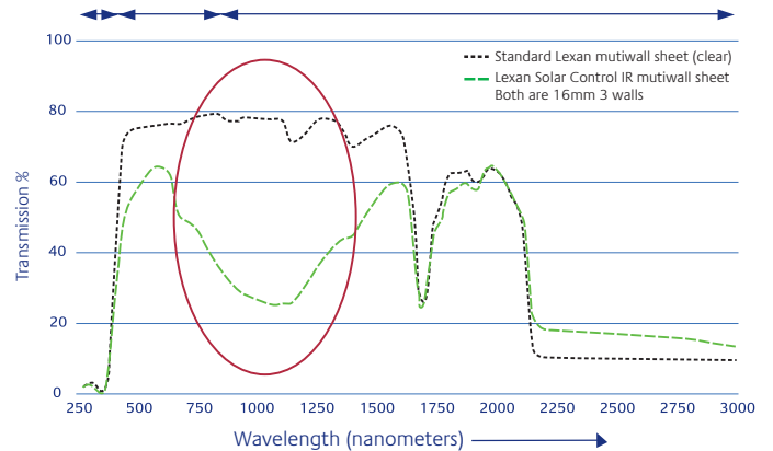
Figure 10: Lexan Solar Control IR sheet selectively blocks the near infra-red region of the light, therefore reduces the heat build up.
